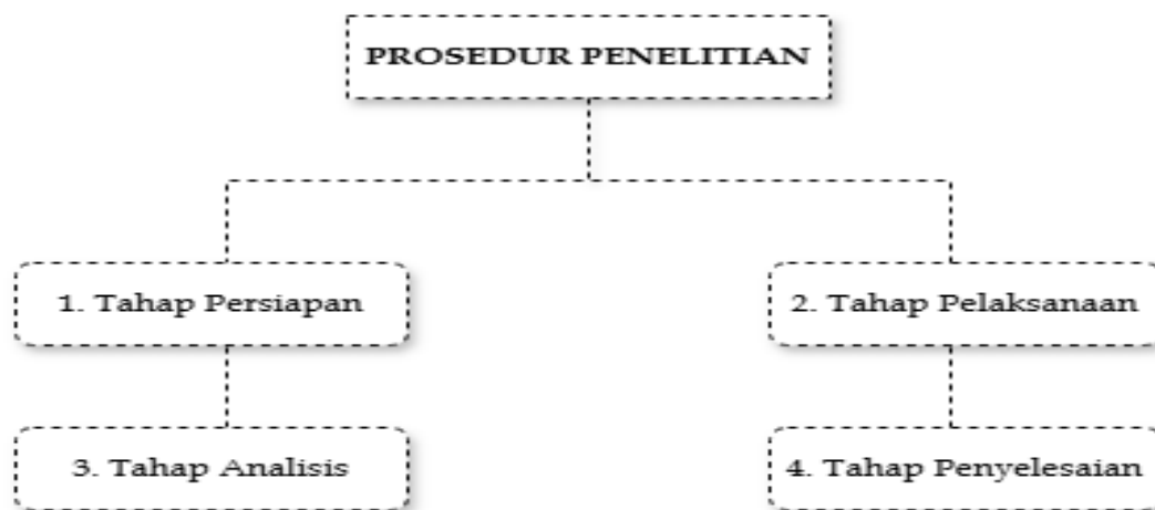
Diagram 1. Prosedur Penelitian
